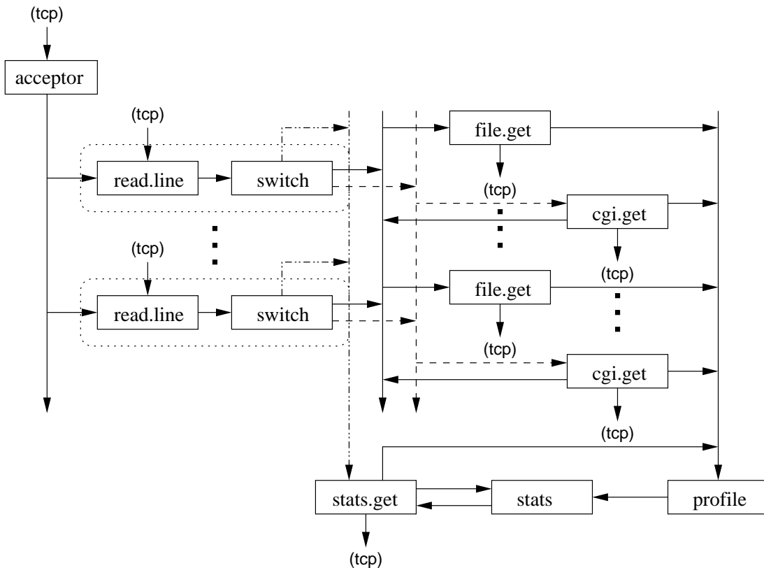
Figure 11: Network diagram for the occam web-server
