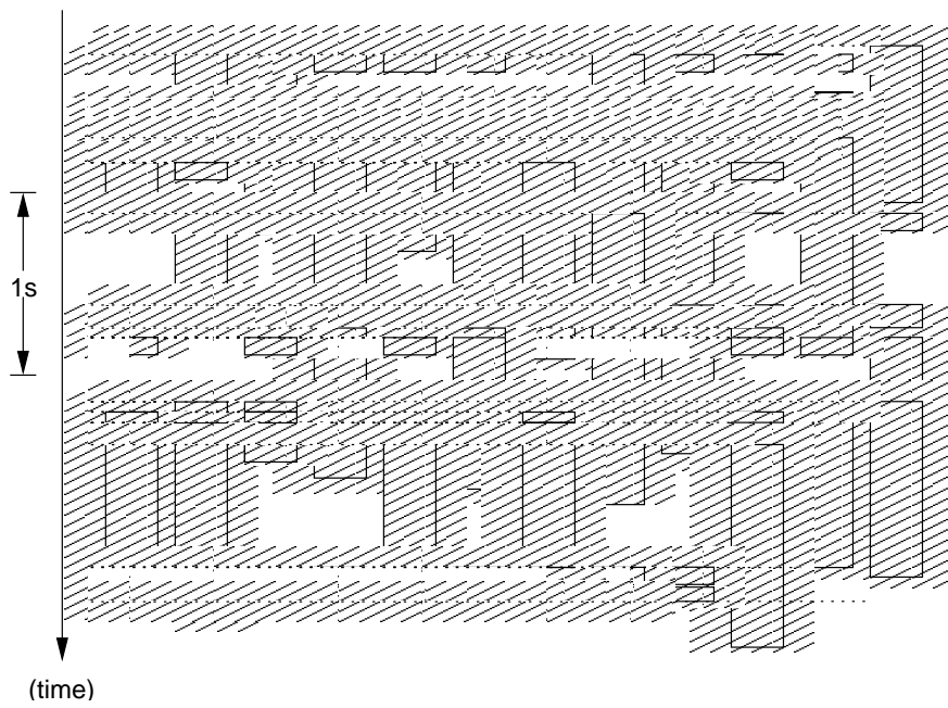
Figure 10: Execution profile of blocking system calls with ob (occam benchmark) showing the 'active' time of each clone
